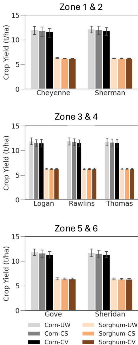
Fig. 9. Predicted annual crop yield for corn and sorghum during synthetic drought simulation under UW, CS, and CV irrigation scenarios. Error bars represent the crop yield RMSE values from the bias-corrected models.
