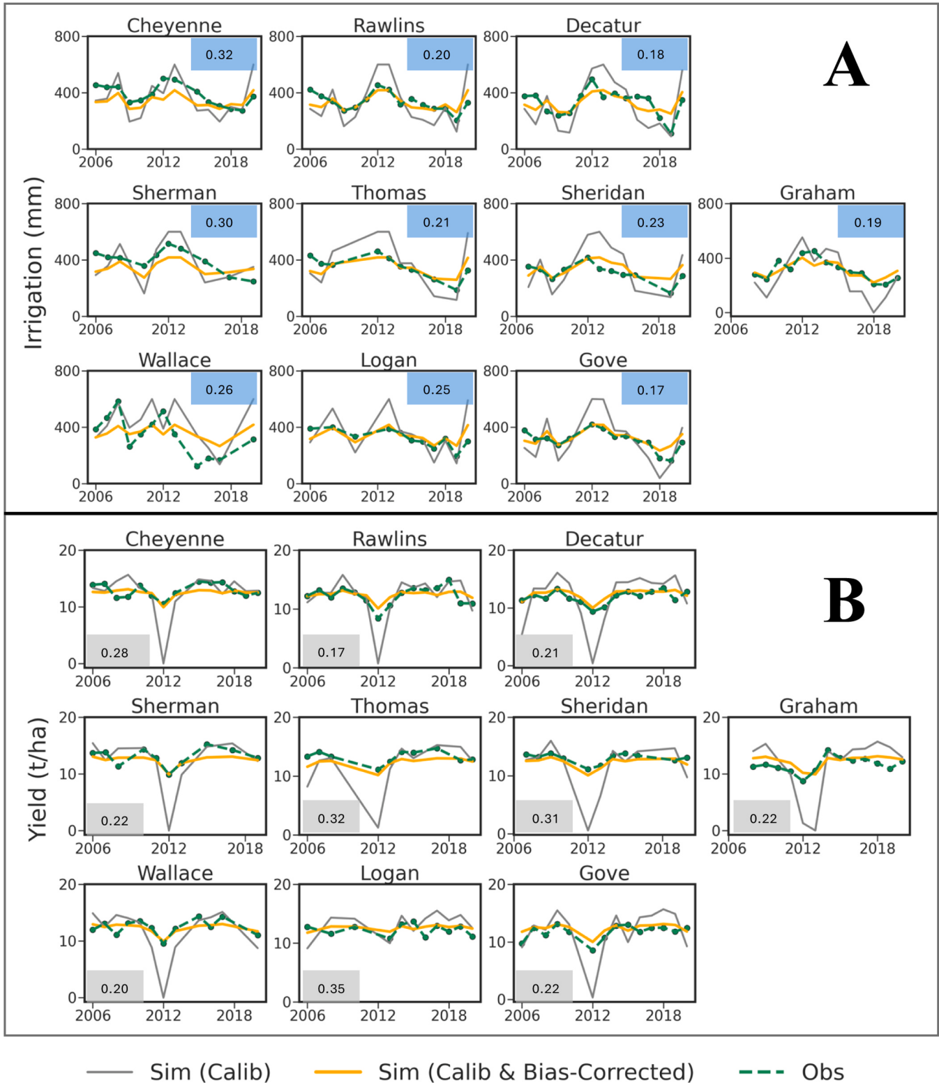
Fig. 6. Comparison of observed, calibrated and bias-corrected irrigation and yield for corn over the 2006–2020 period for each county in the study domain. The blue and gray boxes show the bias-corrected NRSME values for irrigation and crop yield, respectively. The panels are arranged based on the location of the counties (Fig. 1).
