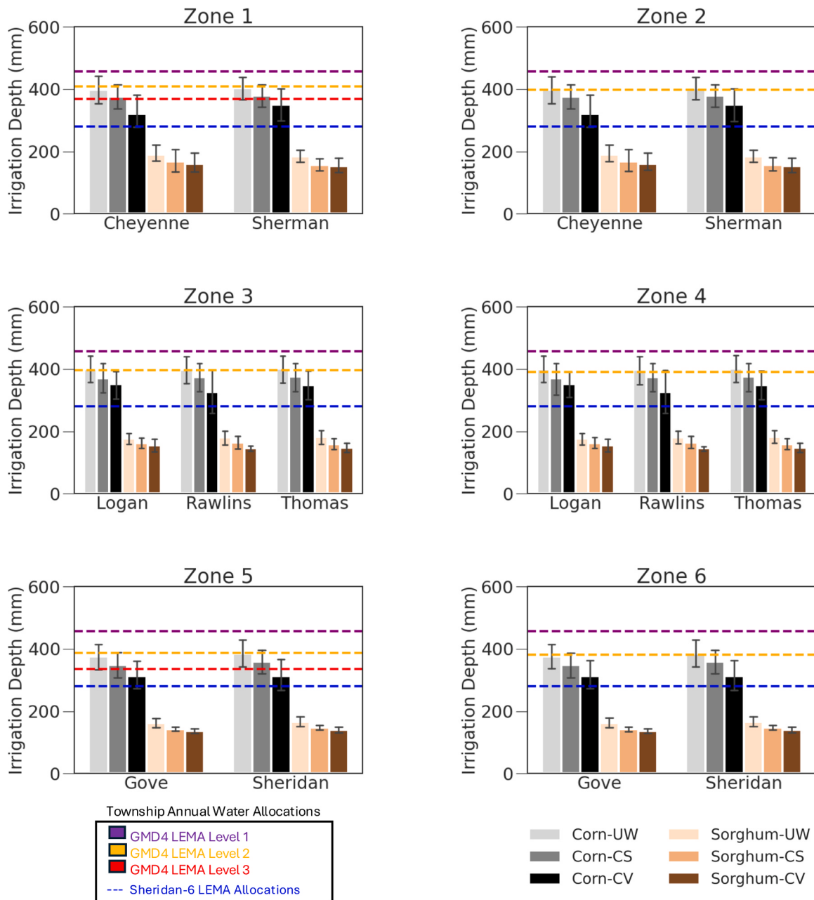
Fig. 8. Predicted annual irrigation depths for corn and sorghum during synthetic drought simulation under UW, CS, and CV irrigation scenarios. The horizontal lines represent the GMD-4 LEMA allocations (Level 1–3) in the six zones within the GMD-4 LEMA shown in Fig. 2. The blue line represents the Sheridan-6 LEMA annual allocation based on the 55 in./5-year LEMA cycle allocation. Error bars represent the irrigation RMSE values from the bias-corrected models.
