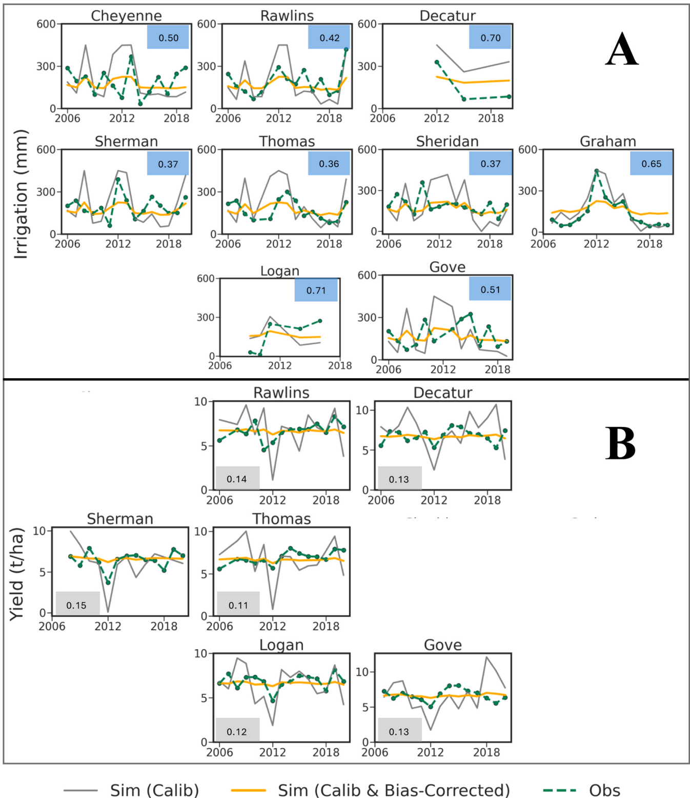
Fig. 7. Comparison of observed, calibrated and bias-corrected irrigation and yield for sorghum over the 2006–2020 period for each county in the study domain. The blue and gray boxes show the bias-corrected NRSME values for irrigation and crop yield, respectively. The panels are arranged based on the location of the counties (Fig. 1).
